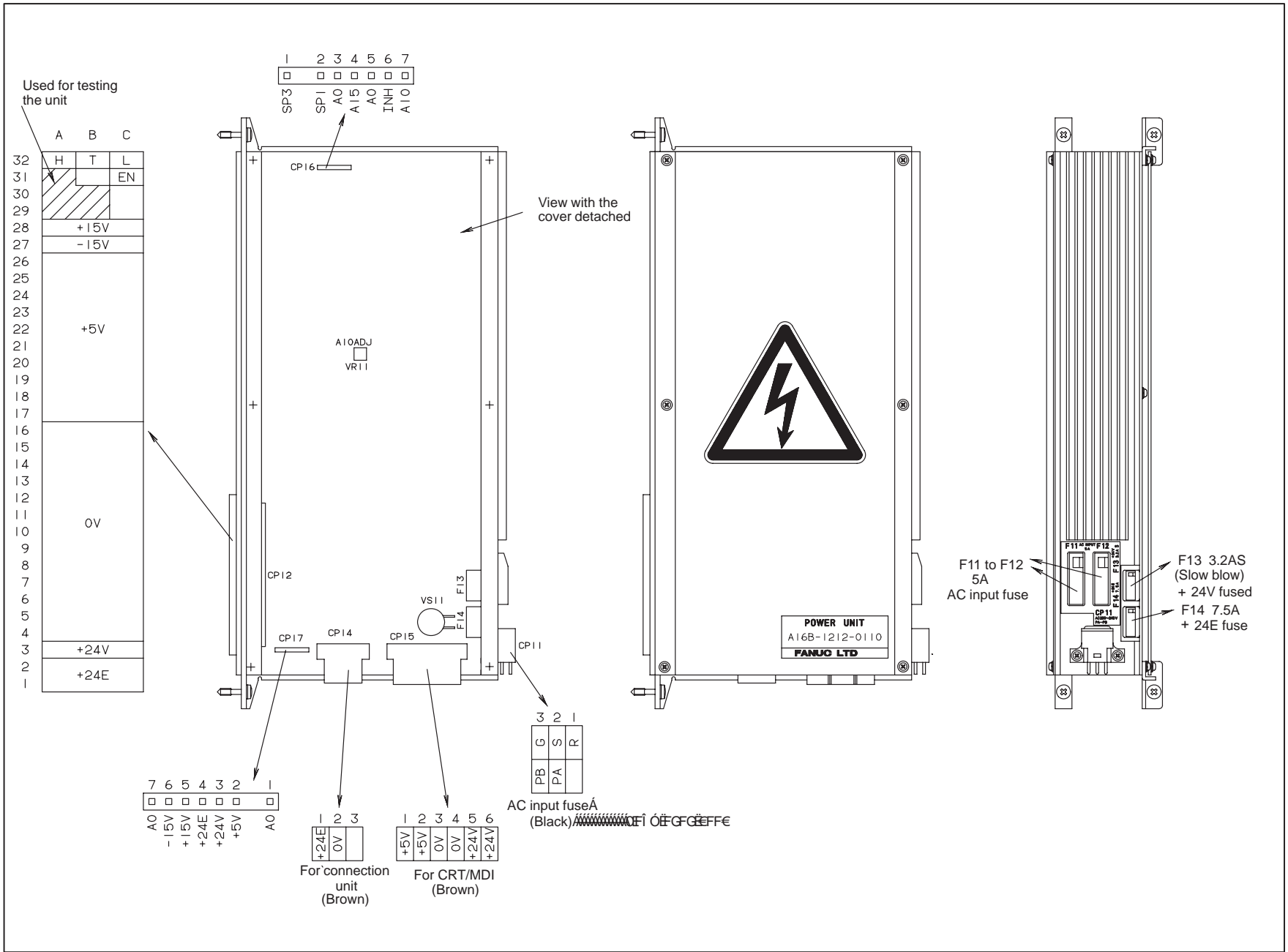
Fig.2.7.2(a) Power supply unit B2 external diagram
