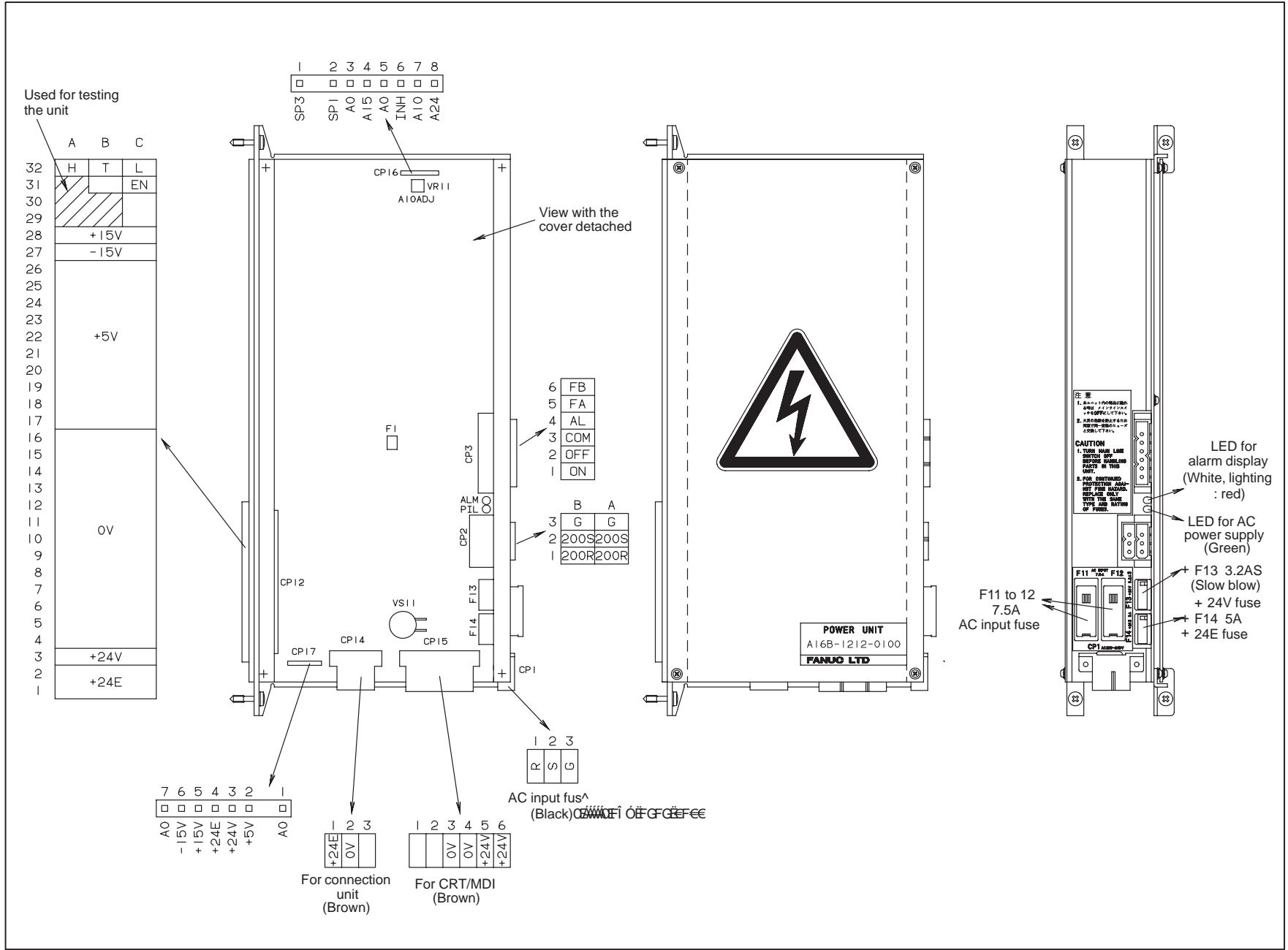
Fig.2.7.3(a) Power supply unit A1 external diagram
